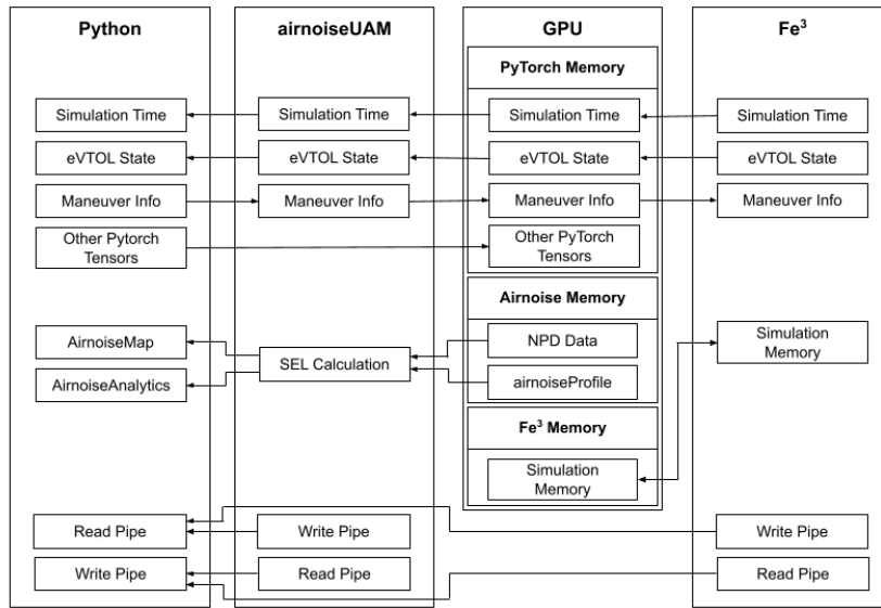
Figure 7. —Shared memory and inter-process communication between Python and Fe 3 processes for noise-minimizing configuration (Ref. 25).
