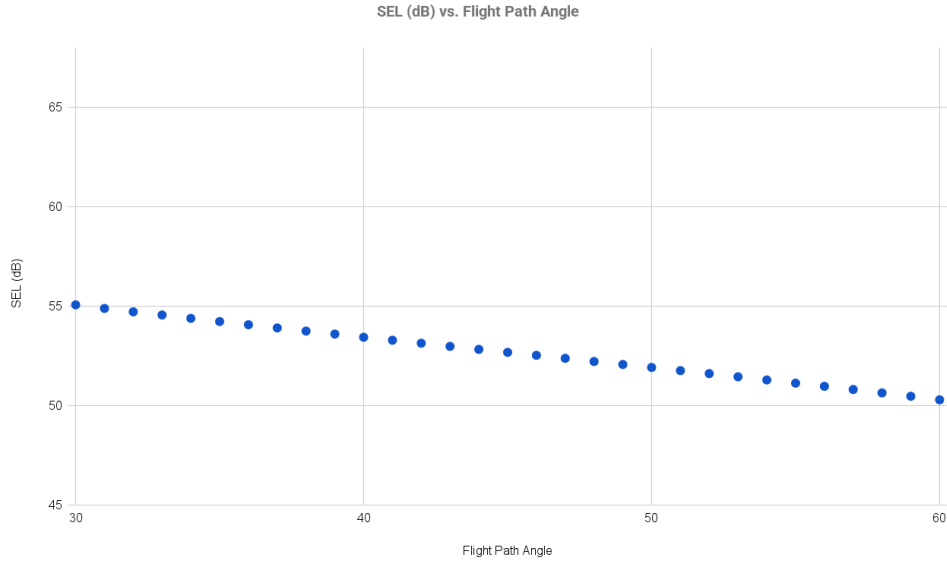
Figure 9. —Estimated SEL vs. Flight Path Angle (Steady State Climb)
