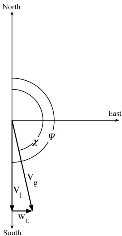
Figure 3. —Navigation frame geometry showing wind vector W_E , airspeed vector V_I , ground speed vector V_g , and angles \psi (heading) and \chi (track).
