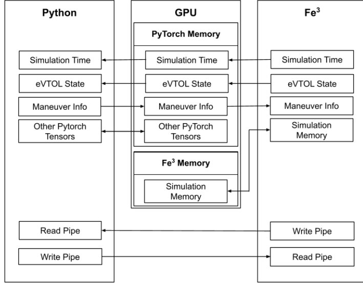
Figure 6. —Shared memory and inter-process communication between Python and Fe 3 processes for energy-optimization configuration (Ref. 25).
